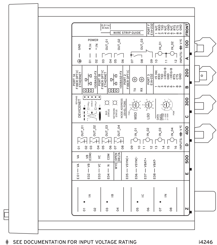
(B) Side-Panel Input and Output Designations
