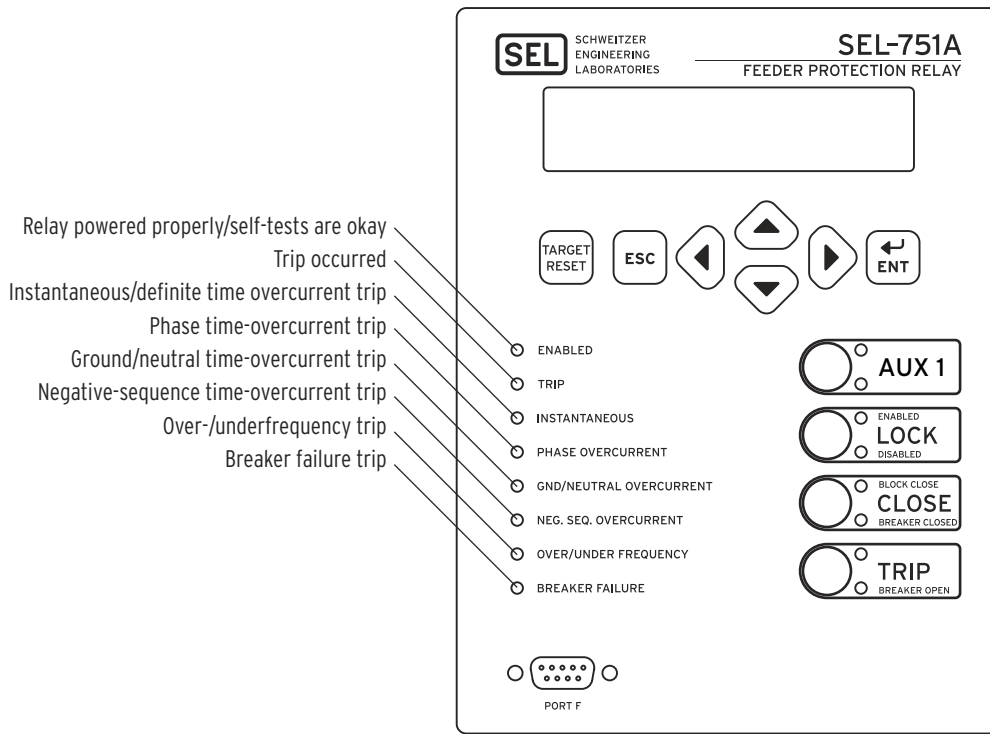
Figure 14 Front Panel With Default Configurable Labels
