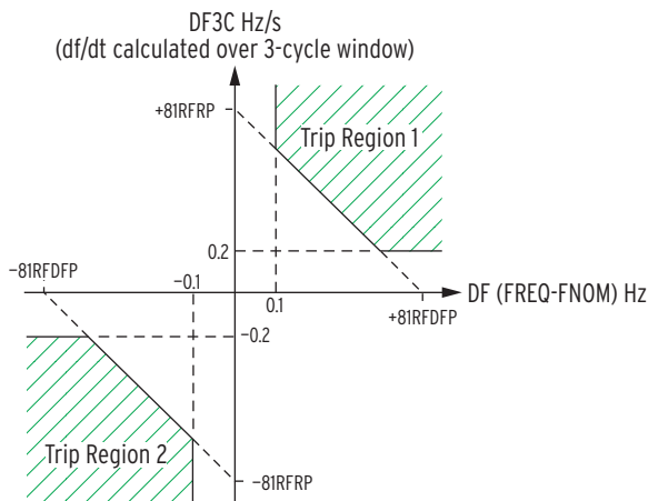
Figure 3 81RF Characteristic
