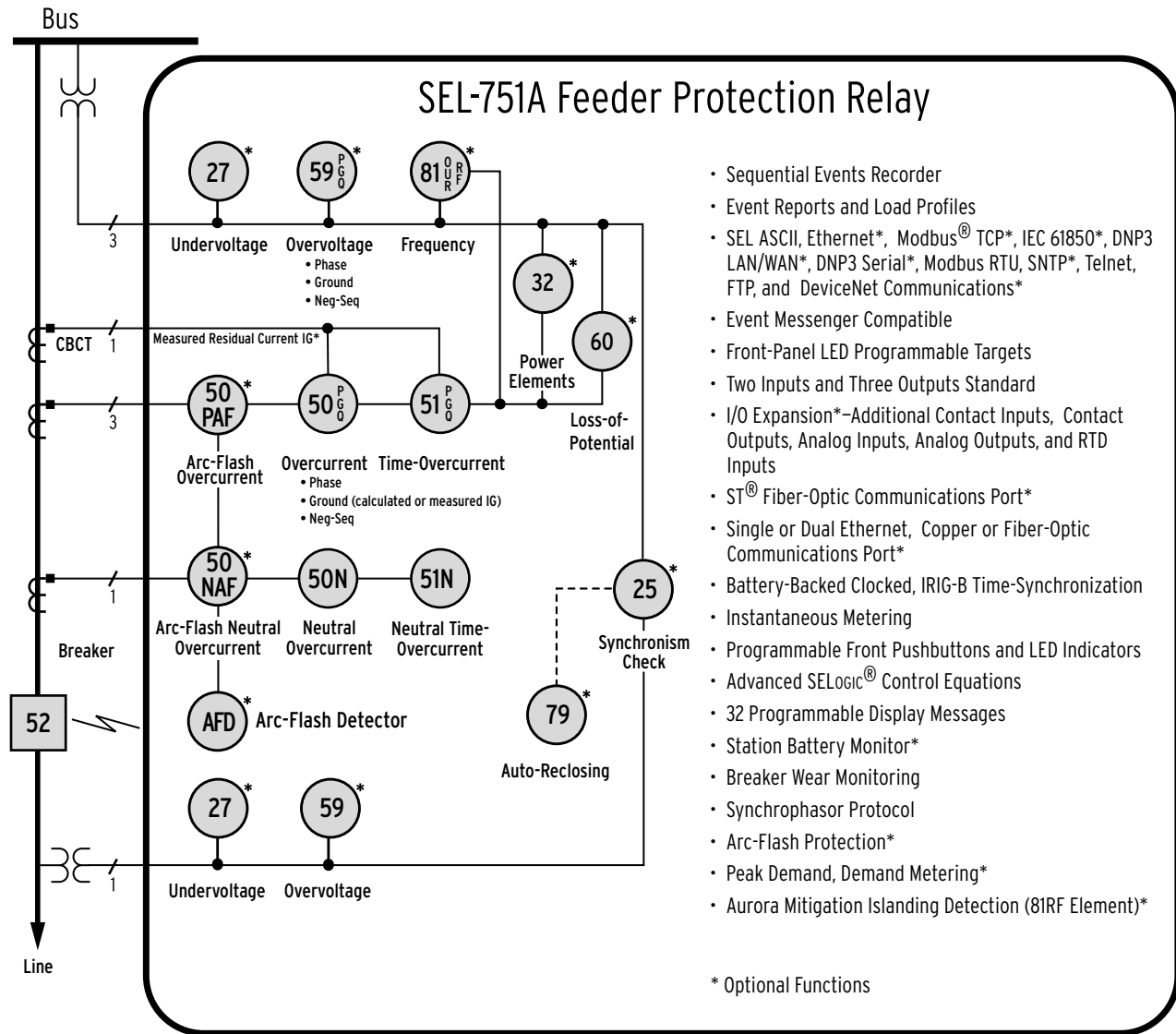
Figure 1 Functional Diagram
